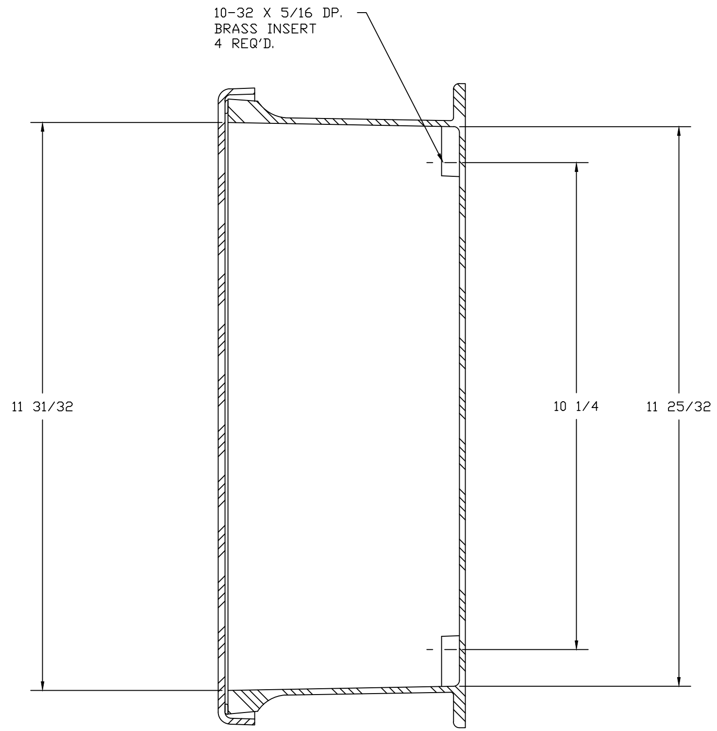
SECTION B-B
