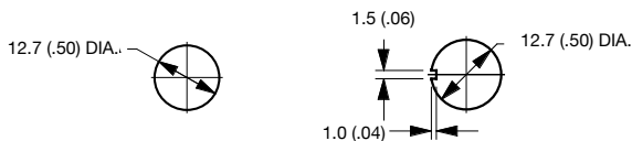
Mounting Hole
