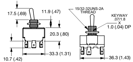
17 Amp, 4 Pole
