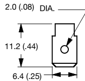
1/4" Q.C. Terminal
